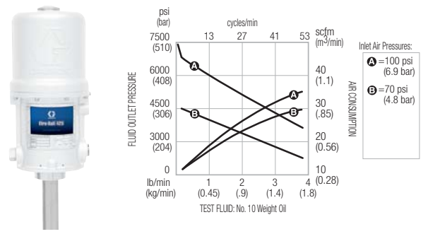
Fire-Ball 425, 10:1 Performance
