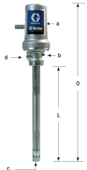
LD Series 181 kg Drum
